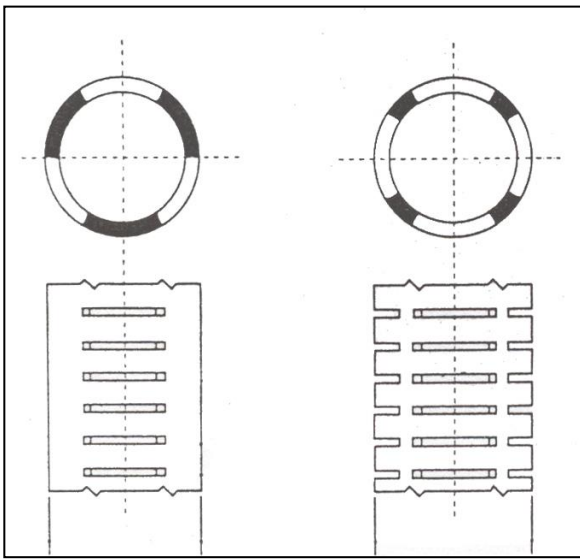
Pic. 2 Section image of cuts made on three and four sides
